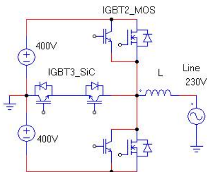
Fig. 7: high voltage NPC
