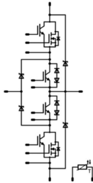
Fig. 5: NPC topology as integrated in the P969-F power module
