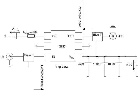
Fig. 1: Test Circuit for Electrical Characteristics and S-Parameter
